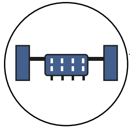
IceCube-Labor
